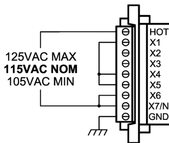
115VAC HOOKUP
