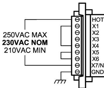
230VAC HOOKUP
