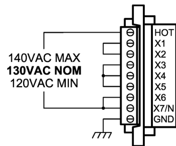
130VAC HOOKUP
