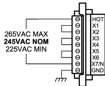
245VAC HOOKUP
